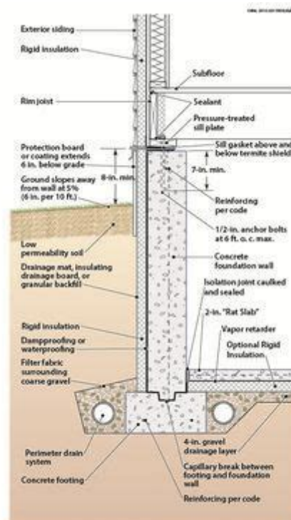
Figure 3-15: Concrete Crawlspace Wall with Exterior Insulation
